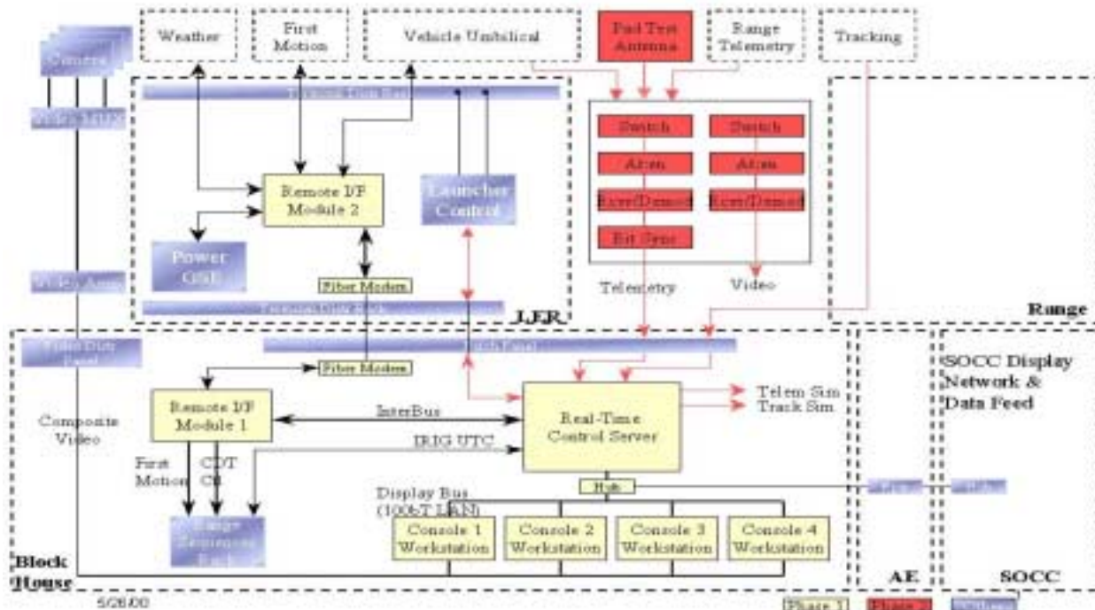
Launch control system architecture, comprised of distributed subsystems connected with standard interfaces, operating systems, and data visualization tools.
